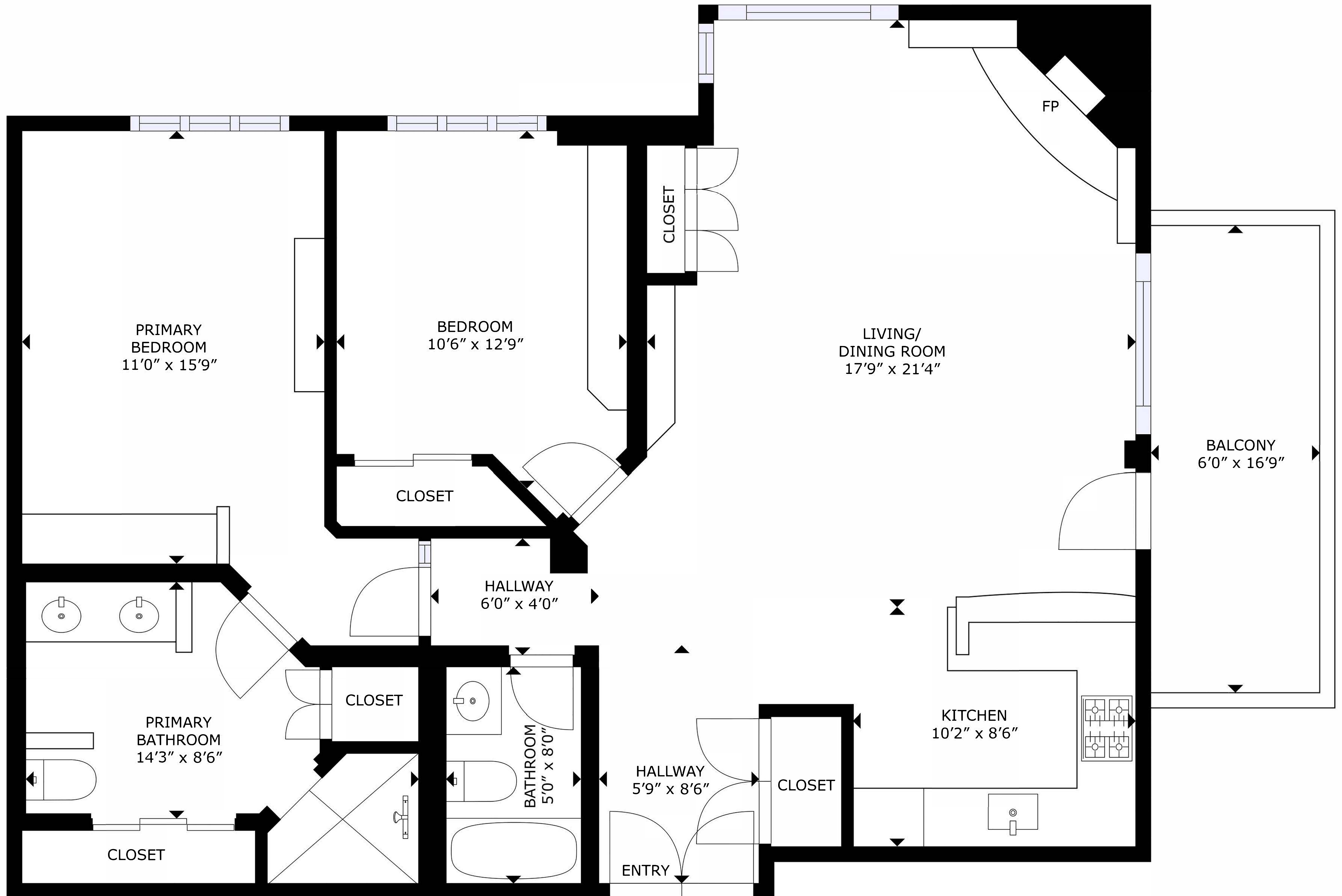
FLOOR PLAN
