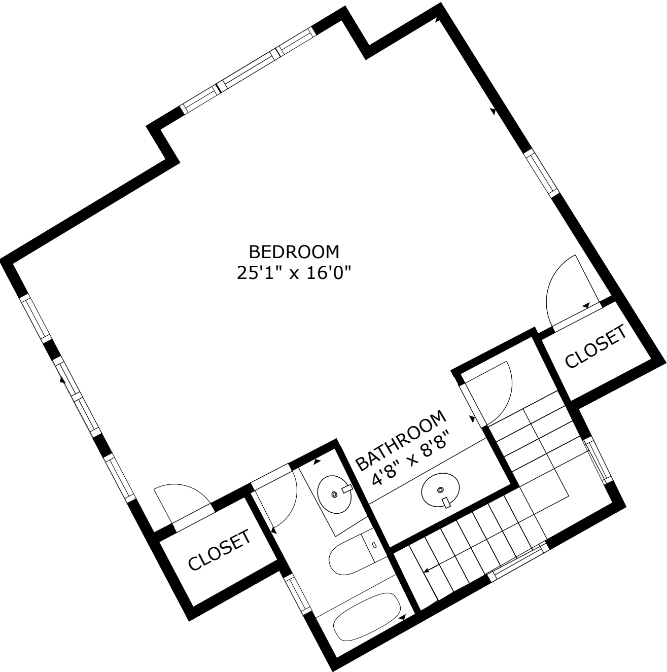
FLOOR 3
