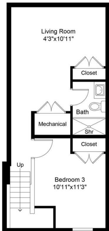
BASEMENT PLAN
